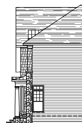
PARTIAL RIGHT SIDE ELEVATION ELEVATION #8A 12-10-19
