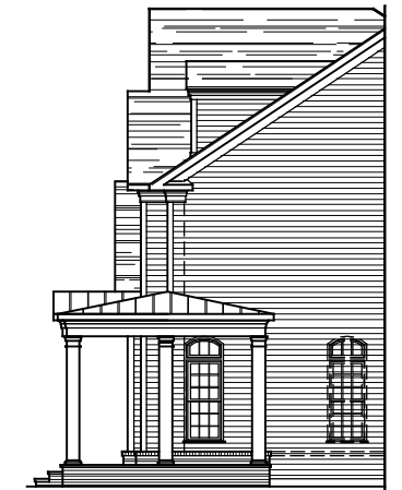
PARTIAL RIGHT SIDE ELEVATION ELEVATION #4C 12-10-19
