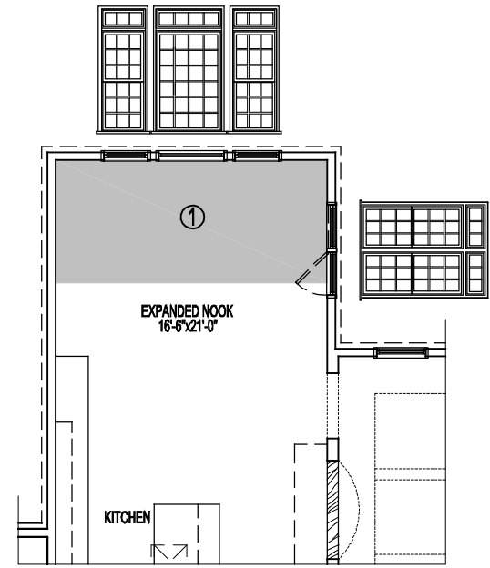
PARTIAL FIRST FLOOR PLAN
