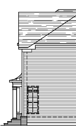
PARTIAL RIGHT SIDE ELEVATION ELEVATION #6A 12-10-19
