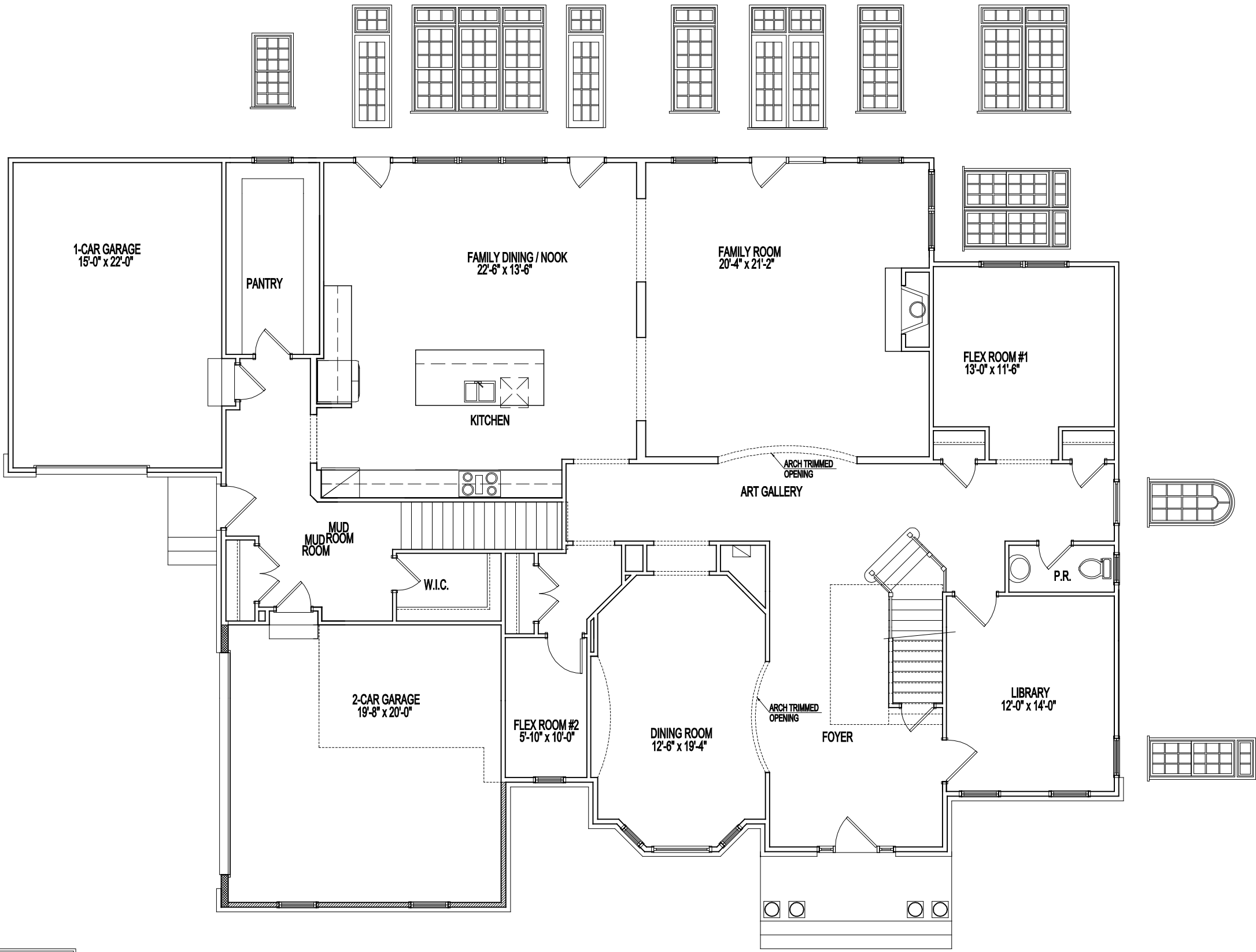
STANDARD FIRST FLOOR PLAN
