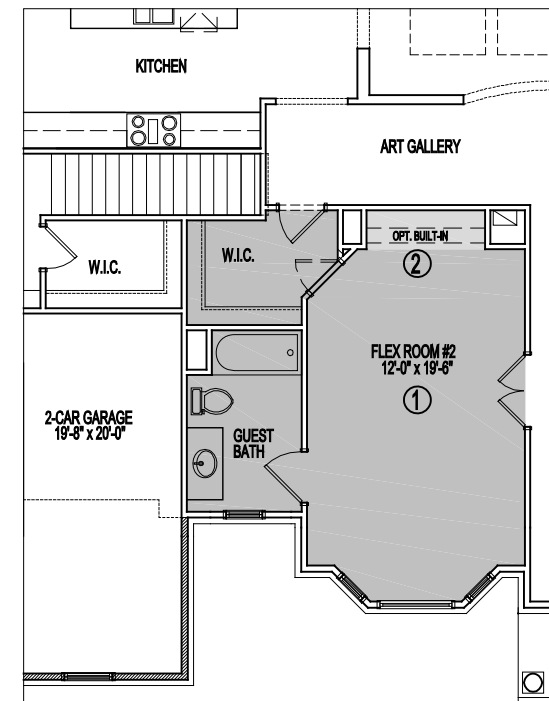
PARTIAL FIRST FLOOR PLAN
