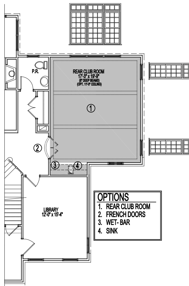
PARTIAL FIRST FLOOR PLAN
